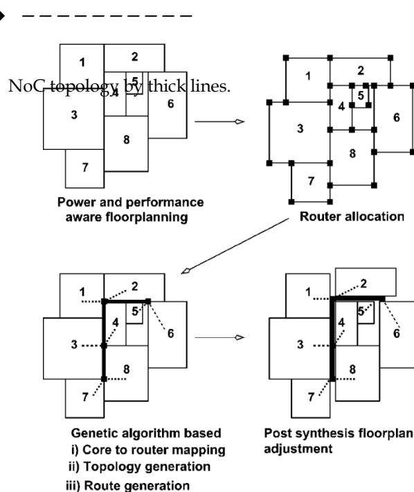
Fig.1 Design Flow for Synthesis of NoC
