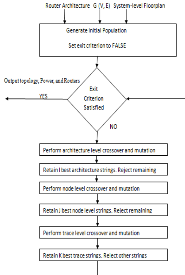
Fig. 3 GA flow for NoC Design
